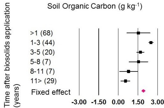
Figure 2 : Mean differences in SOC concentration as influenced by biosolids application:Effect of time. Numbers of observations in y axis are indicated in parentheses and mean differences are indicated in 95 % confidence intervals.
