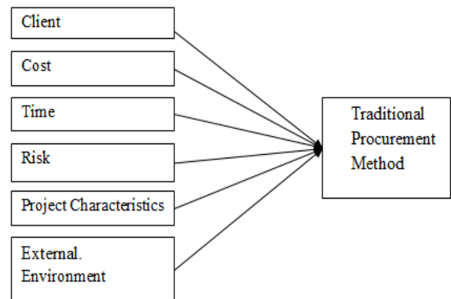
Figure 2: Conceptual Framework
